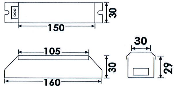
Dimensions (mm)
