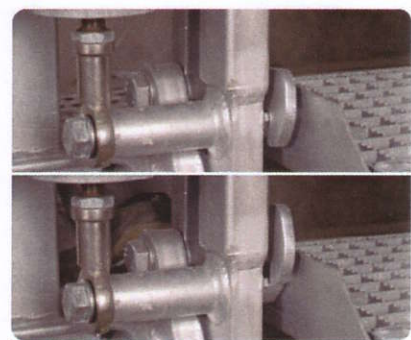
Lock/unlock device
