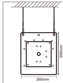
Casing End Cap View
