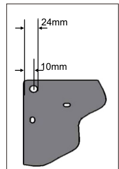
Enlarge Casing End Cap
